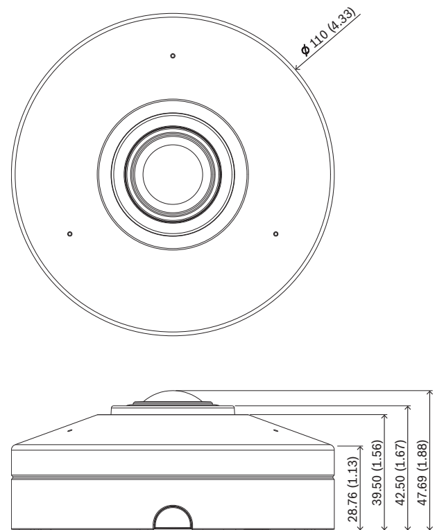
Dimensions in mm (in.)
